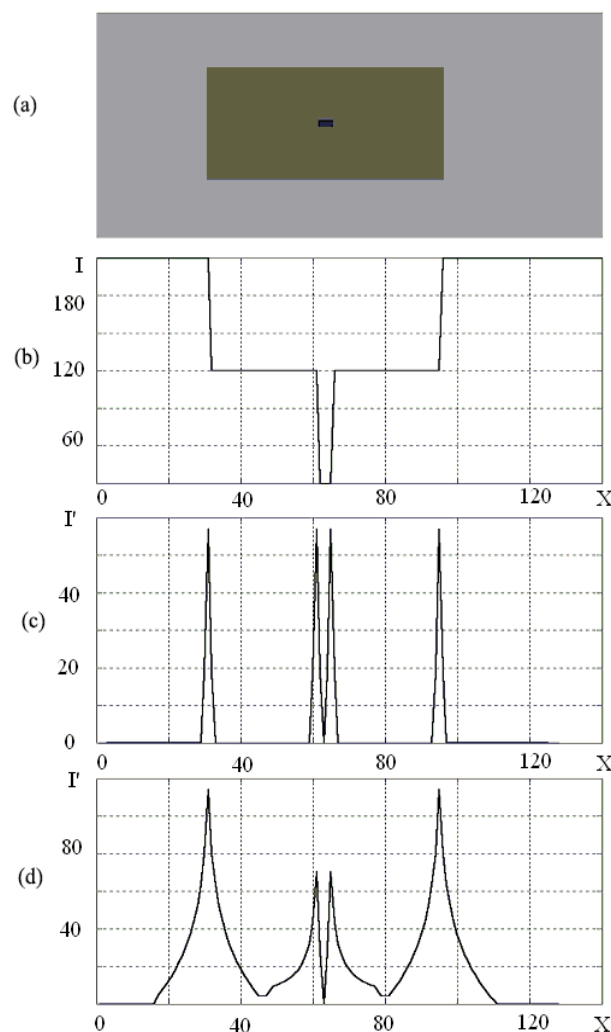
Fig. 1. Modeling results: (a), (b) – test image and its line; (c), (d) – image line in the wavelet transform domain for Gauss Wavelet Transform on different scales s_2 > s_1 Source: compiled by [15]
