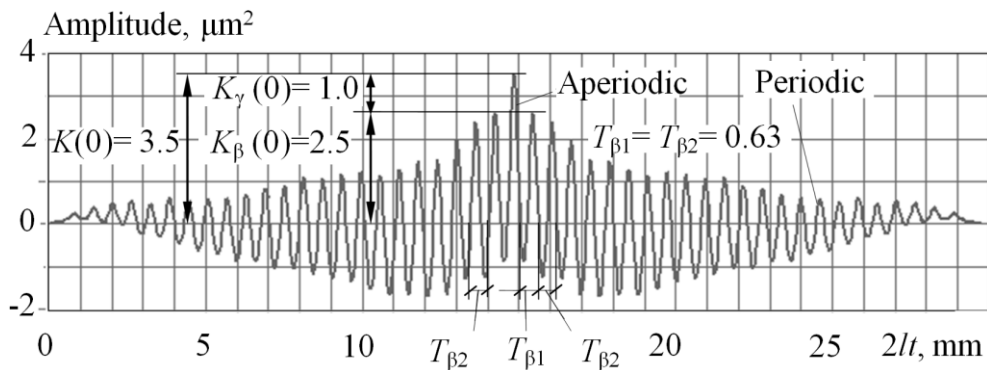
Fig. 8. Correlogram of sample 5.1
