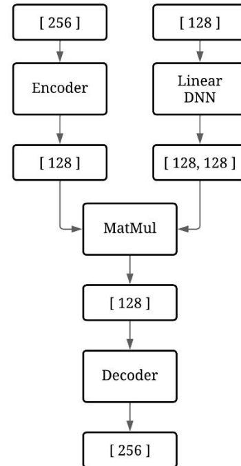
Fig. 7. Proposed method. Predictor model
